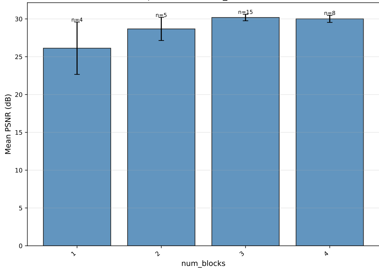
Mean PSNR per value of num_blocks — SRFormer
